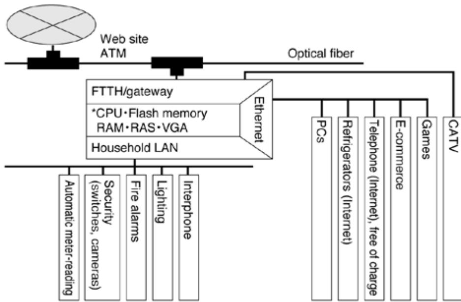
Fig. 9 A typical implementation of the " SMS-10 " as an FTTH gateway
