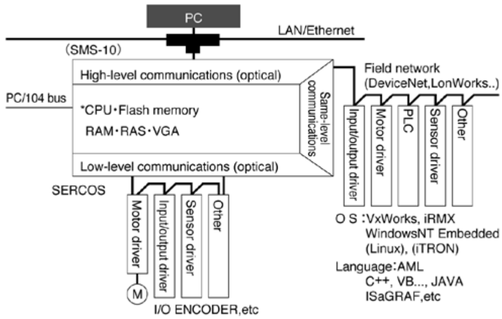
Fig. 8 Interface configuration of " SMS-10 "
