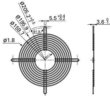
Outlet side
