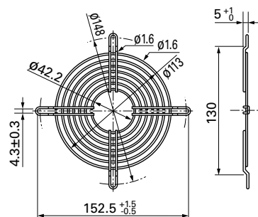
Outlet side
