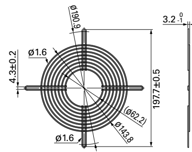
Outlet side
